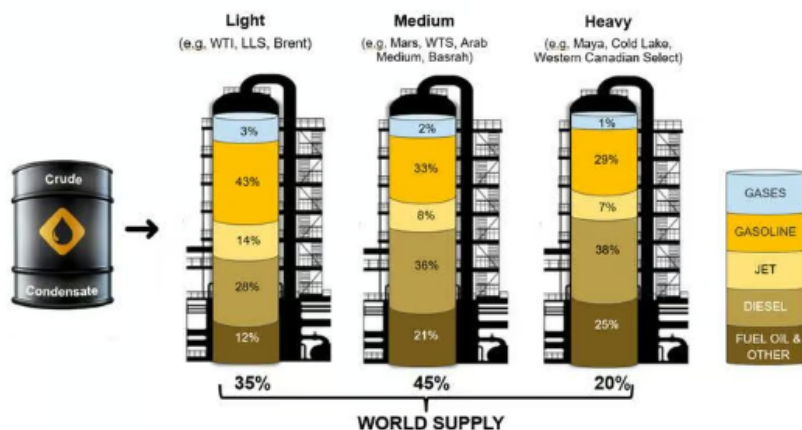
Figure 1: Typical product yields by crude grade
