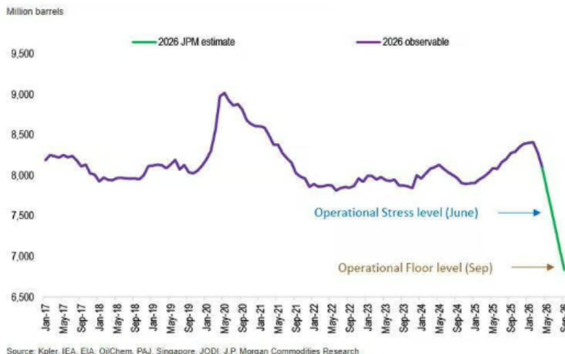
Figure 2: Global oil inventories
